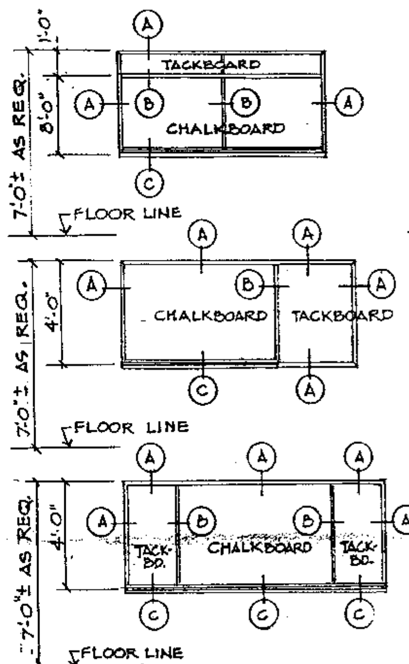
TYPICAL ELEVATIONS
